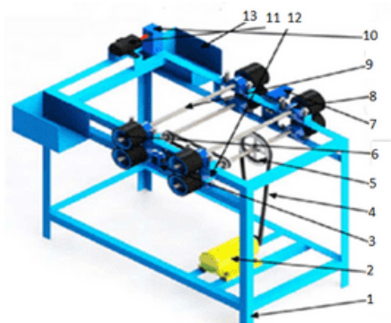
Gambar 1. Model rancangan alat pengirat bambu mekanik
